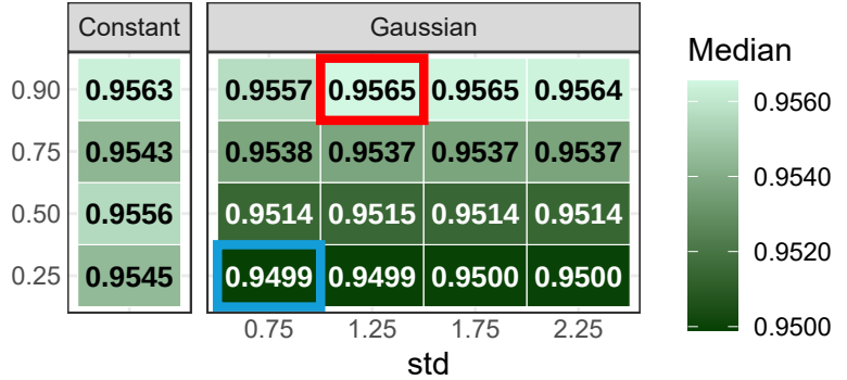
Jaccard
