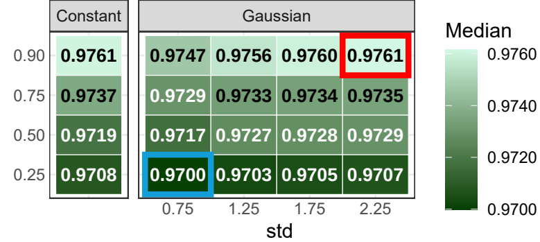
Specificity
