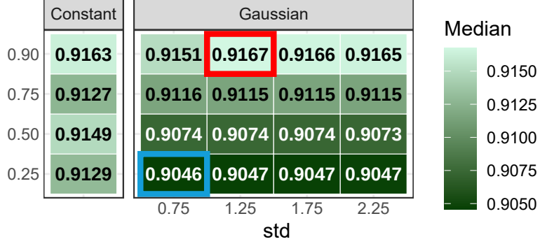
Sensitivity
